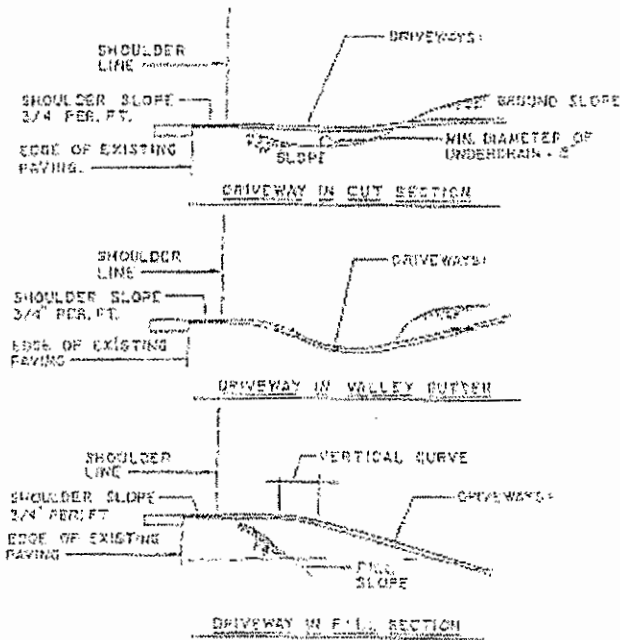
TYPICAL CROSS-SECTIONS OF DRIVEWAYS WHERE CONCRETE CURBS AND SIDEWALKS DO NOT EXIST.
